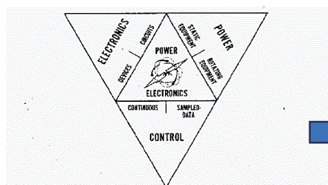
Fig. 1. Power electronics: interstitial to all major disciplines of electrical engineering.
